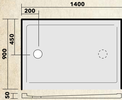
ST1490 3 Sided Left hand/Right hand centre waste
