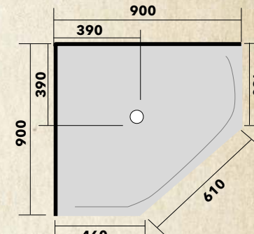
ST4529090 Angle Corner - Centre Waste
