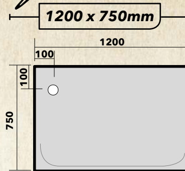
STF41275 Left rear/right front waste, 4 Lip tray - suit either 3 Sided Alcove or 2 Sided Corner
