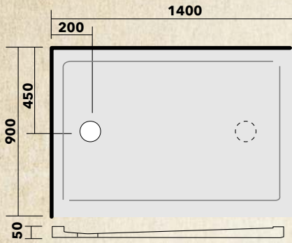
ST1490 2 Sided Left hand/Right hand centre waste
