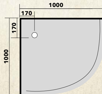
STC1010 Freeflow Corner Waste ONLY
