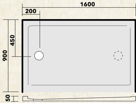
ST1690 3 Sided Left hand/Right hand centre waste
