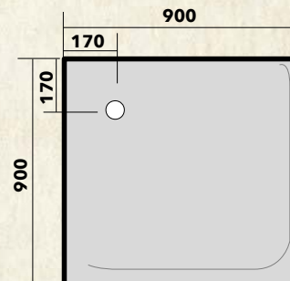
STF39090 3 Sided Alcove Freeflow Corner Waste - Left Rear Position only
