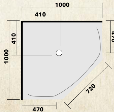
ST4521010 Angle Corner - Centre Waste
