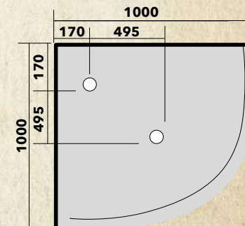
STRR1010 STRC1010 Rear Corner Waste Centre Waste
