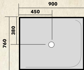
STF49076 Centre Waste - 4 Lip tray Suit either 3 Sided Alcove or 2 Sided Corner
