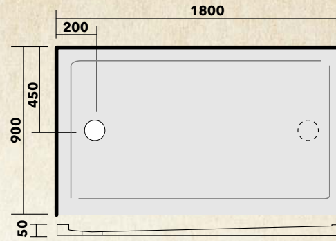
ST1890 2 Sided Left hand/Right hand centre waste
