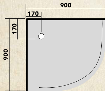
STC9090 Freeflow Corner Waste ONLY
