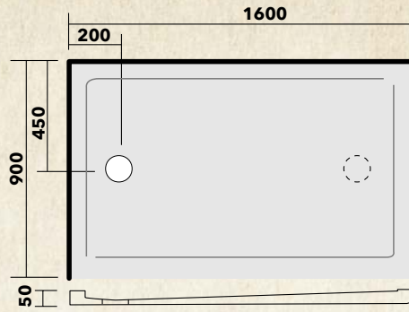
ST1690 2 Sided Left hand/Right hand centre waste
