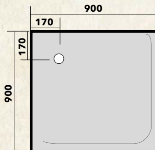
STF29090 2 Sided Corner Freeflow Corner Waste
