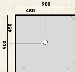
ST39090 3 Sided Alcove Centre Waste
