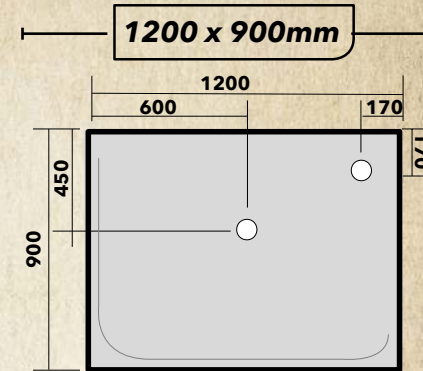
STF41290 Rear right waste - 4 Lip tray ST41290 Centre Waste - 4 Lip Tray Suit either 3 Sided Alcove or 2 Sided Corner
