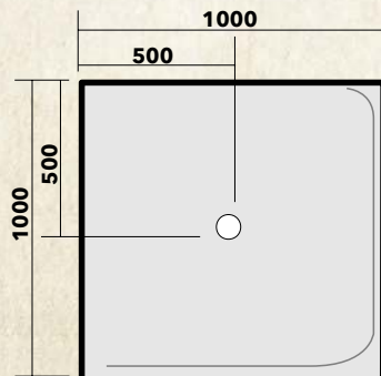
ST31010 3 Sided Alcove Centre Waste
