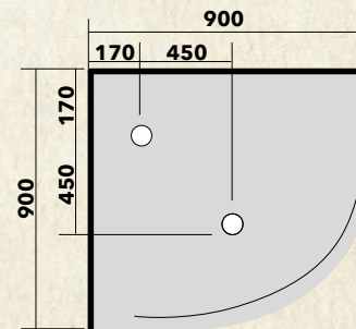
STRR9090 STRC9090 Rear Corner Waste Centre Waste
