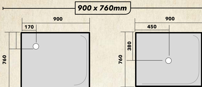
STF39076 3 Sided Alcove Freeflow Corner Waste
