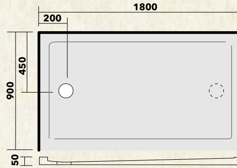
ST1890 3 Sided Left hand/Right hand centre waste
