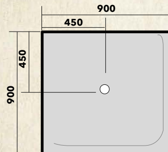
ST29090 2 Sided Corner Centre Waste
